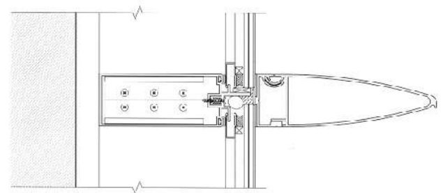
CORTE VERTICAL
