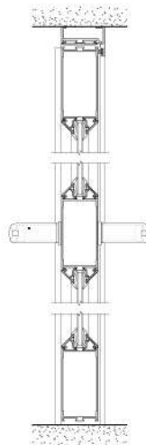
CORTE VERTICAL
