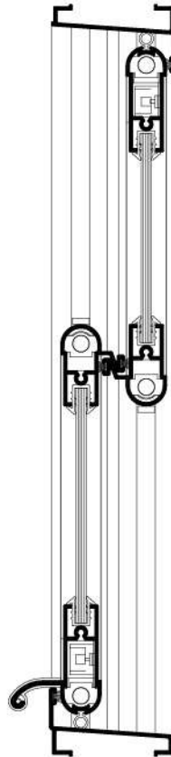
CORTE VERTICAL
