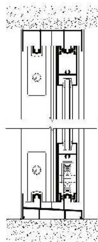
CORTE VERTICAL
