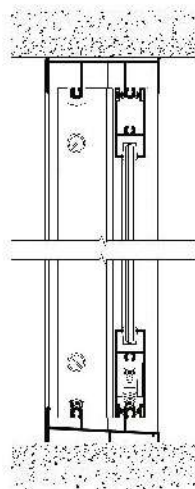
CORTE VERTICAL
