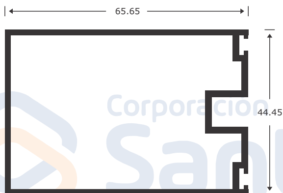
4502 MULLION
